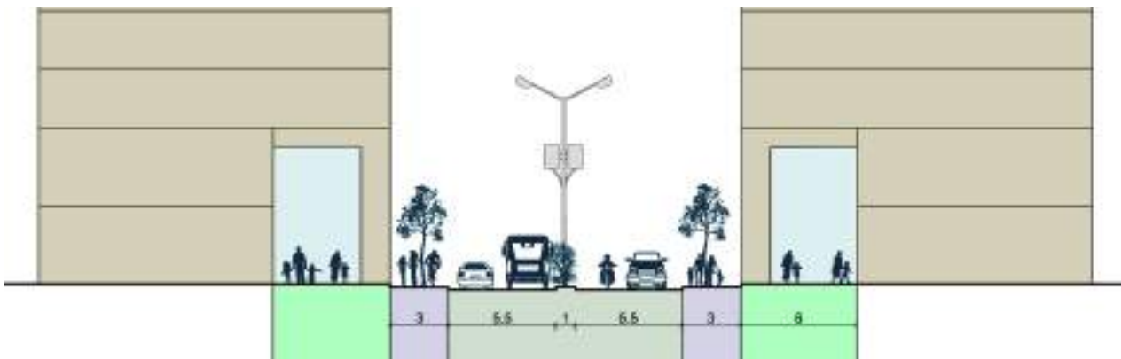
26. 18m ROW - PROPOSED STREET SECTION
